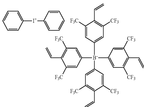
[Chemical Formula 1-1-17]
