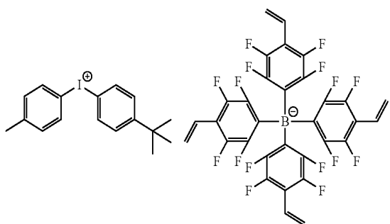
[Chemical Formula 1-1-18]
