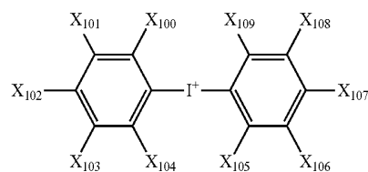
[Chemical Formula 11]
