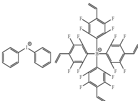
[Compound 4]
