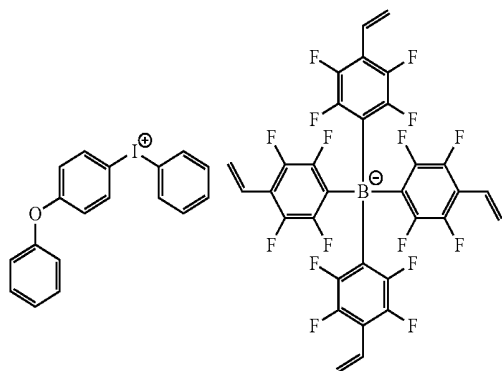
[Chemical Formula 1-1-8]
