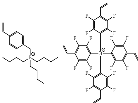
[Chemical Formula 1-2-3]
