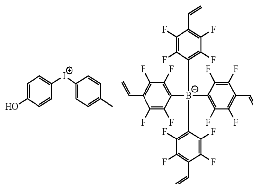
[Chemical Formula 1-1-5]
