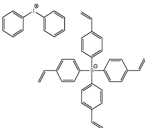
[Comparative Compound 1]
