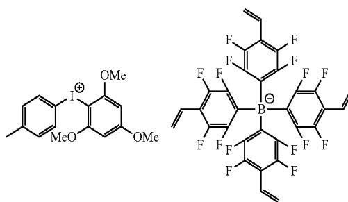
[Chemical Formula 1-1-19]
