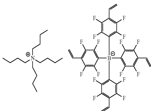
[Chemical Formula 1-4-1]
