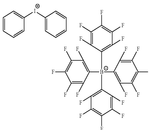
[Comparative Compound 2]
