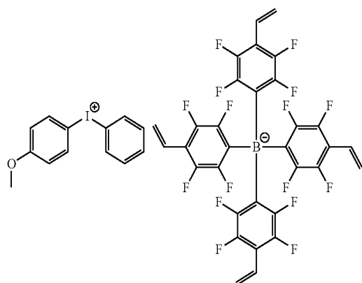
[Chemical Formula 1-1-6]
