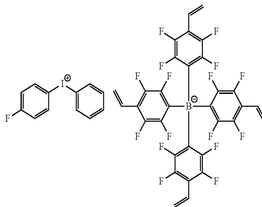
[Chemical Formula 1-1-9]
