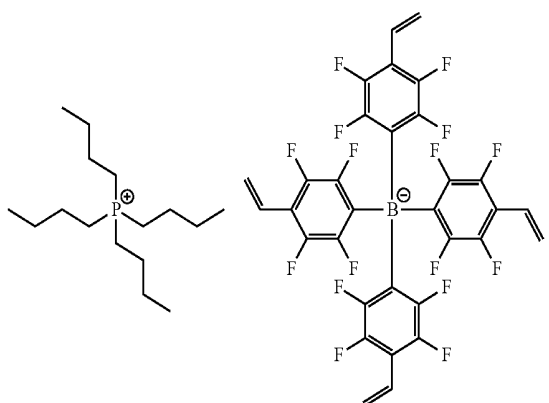
[Chemical Formula 1-2-1]
