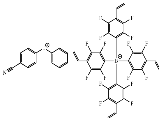
[Chemical Formula 1-1-11]
