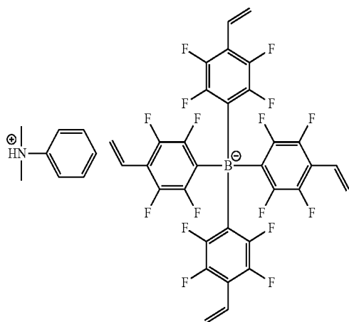
[Chemical Formula 1-3-1]
