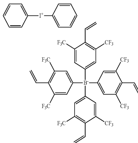
[Comparative Compound 2]
