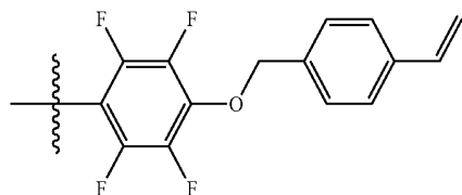
[Chemical Formula 2-9]
