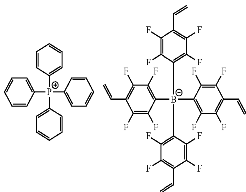
[Chemical Formula 1-2-2]
