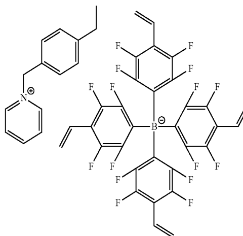
[Compound 3]
