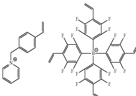
[Chemical Formula 1-5-1]
