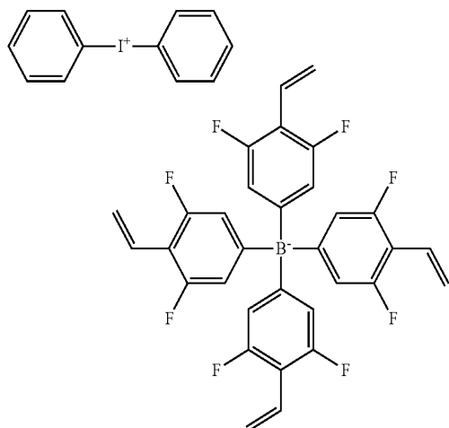
[Compound 2]
