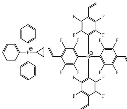
[Chemical Formula 1-5-1]
