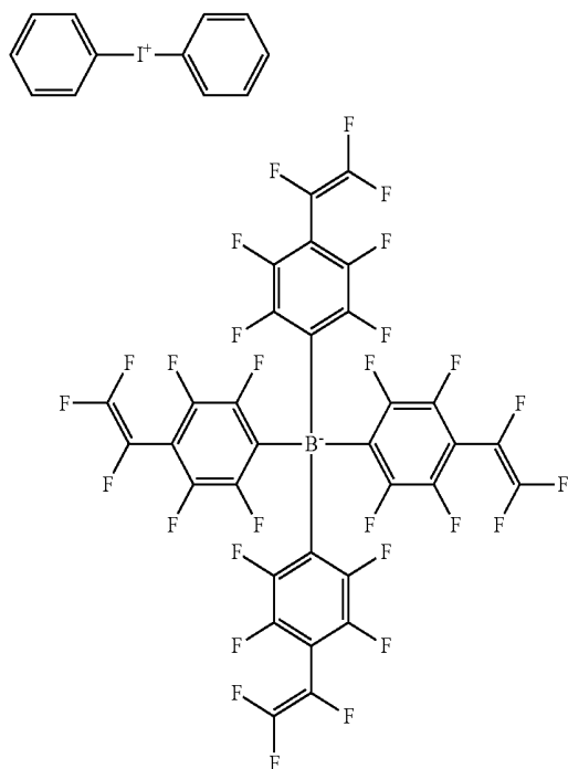
[Chemical Formula 1-1-15]
