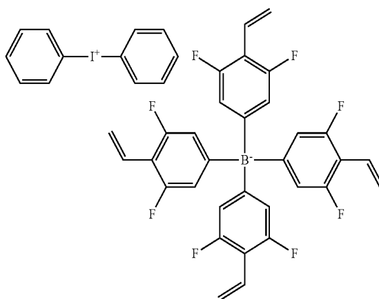
[Chemical Formula 1-1-16]
