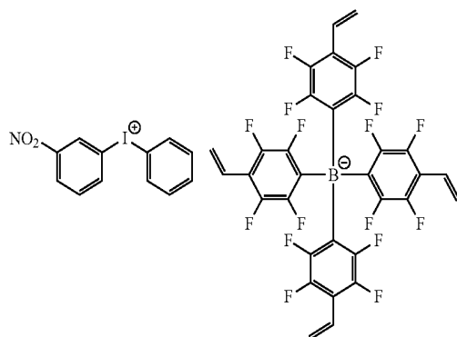
[Chemical Formula 1-1-10]
