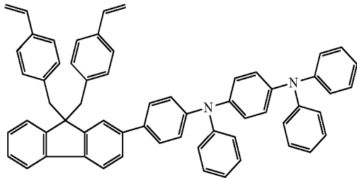
[Compound B]
