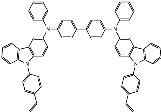
[Compound C]
