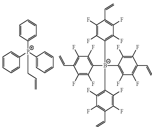
[Chemical Formula 1-2-4]
