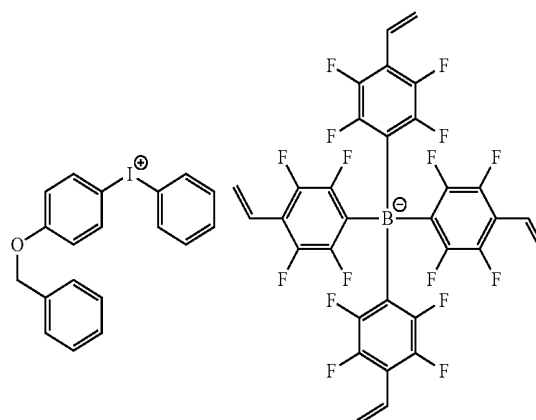
[Chemical Formula 1-1-7]
