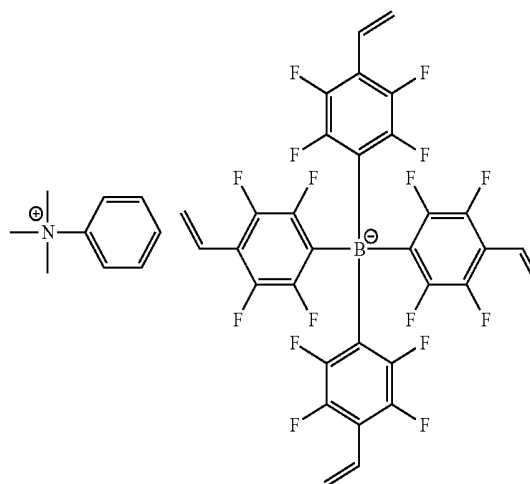
[Chemical Formula 1-3-2]
