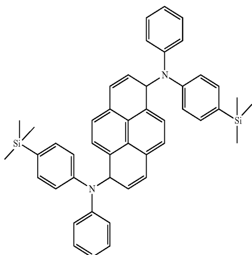
[Compound G]
