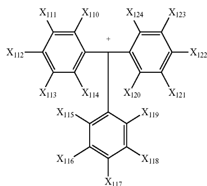
[Chemical Formula 12]
