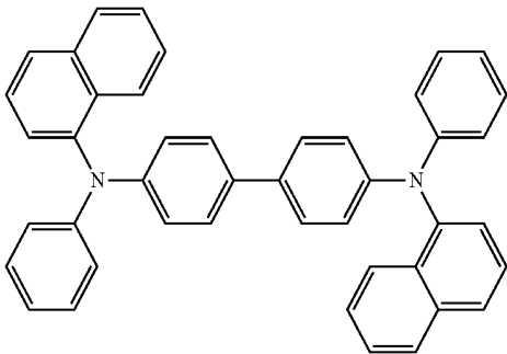
[Compound D]
