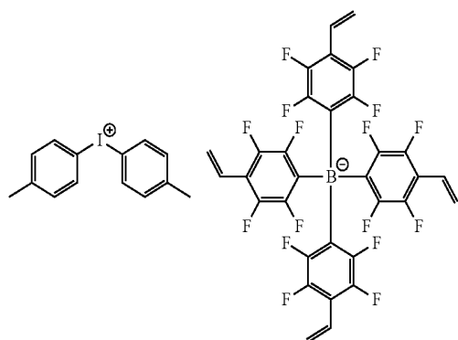
[Chemical Formula 1-1-4]
