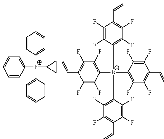
[Chemical Formula 1-2-5]
